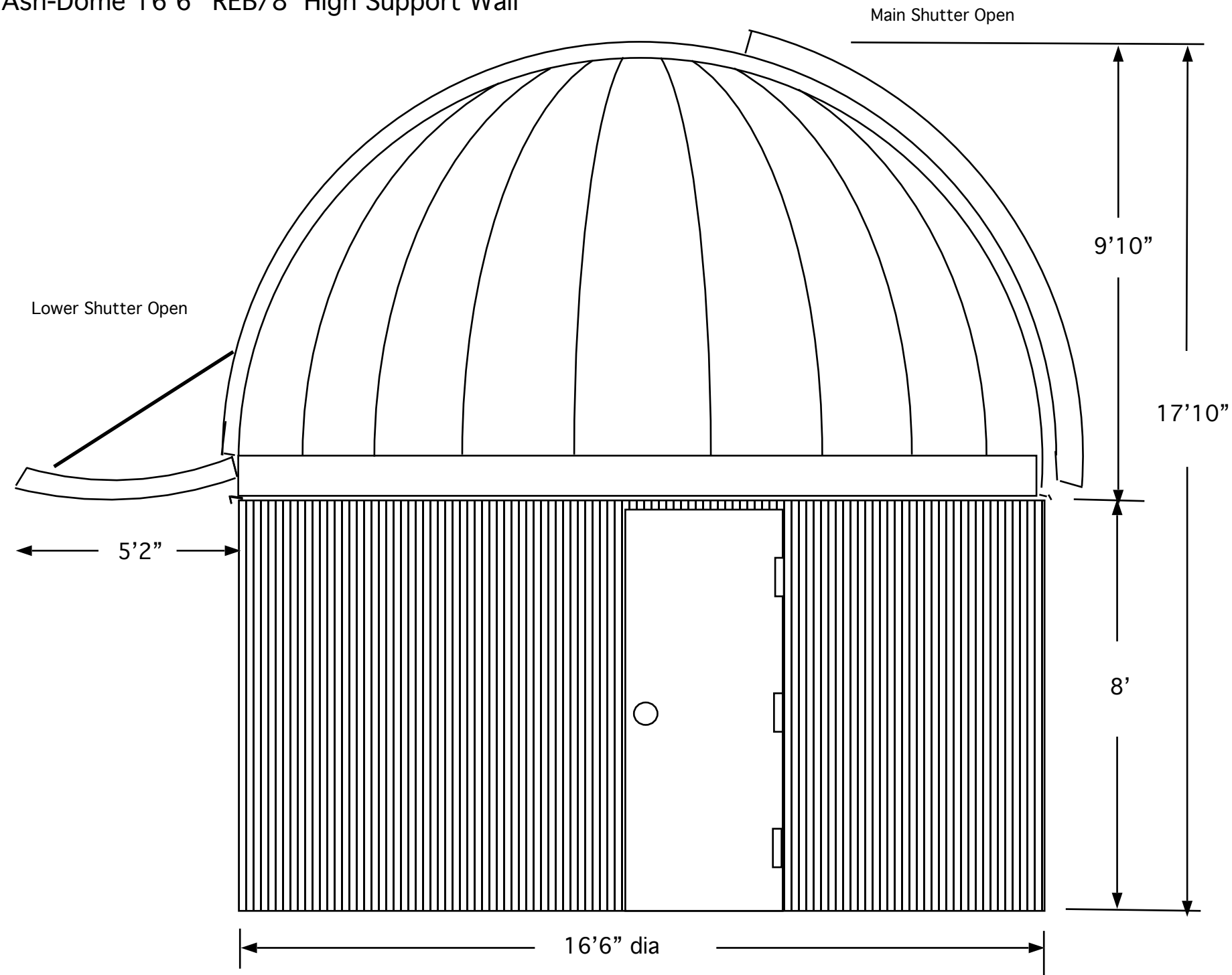
Ash-Dome 16'6" REB/8' High Support Wall
